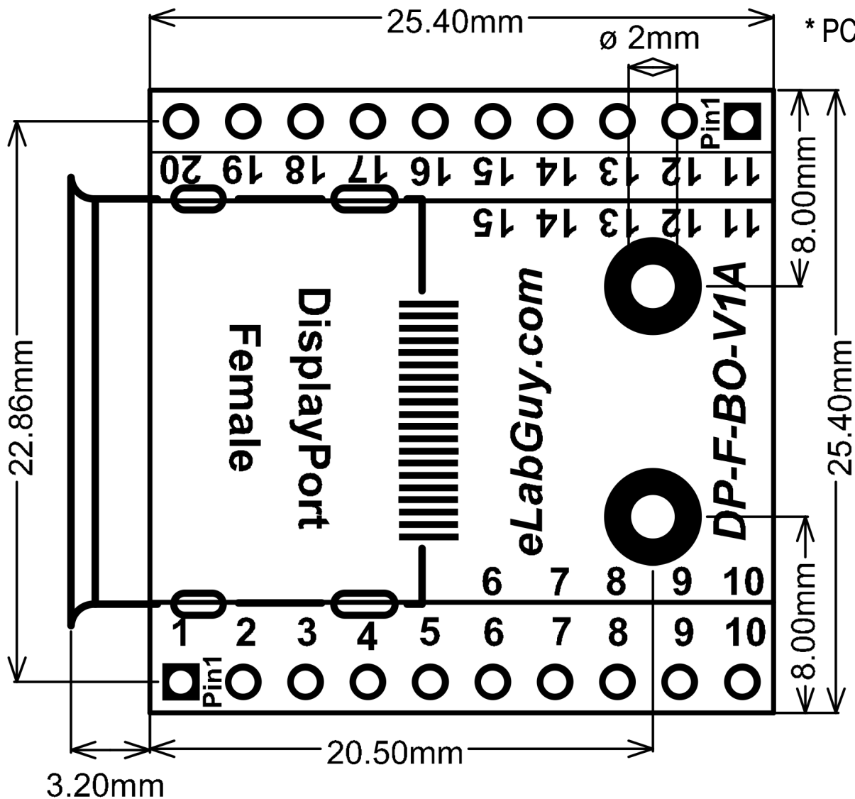
DP-F-BO-V1A PCB outline Drawing
